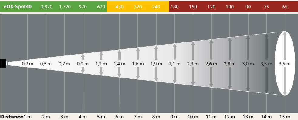
eOX SPOT 40 Illuminance [lux]
