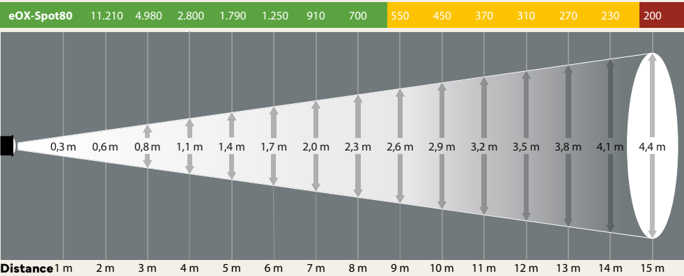
eOX-SPOT 80 Illuminance [lux]
